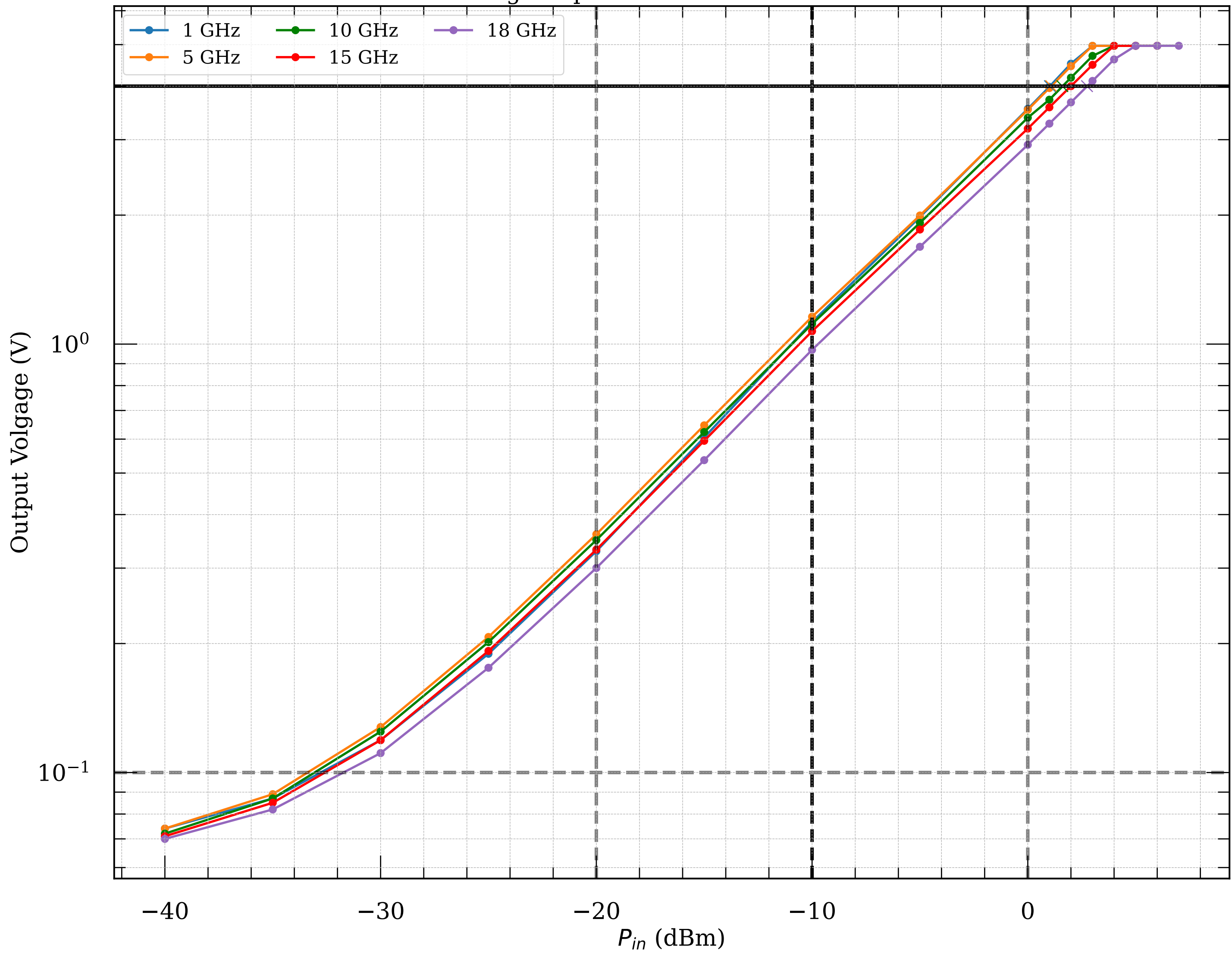
Measured voltage-to-power curve of detector module023v2
